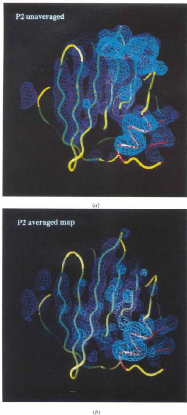
Fig. 2. Results of the template convolution calculations with ESSENS using the unaveraged (a) and the averaged MIR map (b) of P2 myelin (Jones et al. , 1988; Cowan, Newcomer & Jones, 1993). The filtered \alpha -helical scoring maps are shown in cyan, and the filtered \beta -strand scoring maps in magenta. The colouring of the C\alpha trace of P2 myelin is the same as in Fig. 1. The extra features in the unaveraged map represent signal from symmetry-related molecules.
